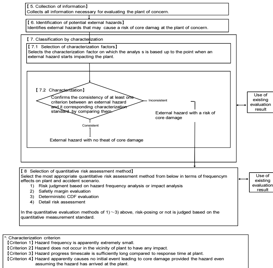
Figure 1 Flow of Selecting Risk Assessment Method for External Hazards
